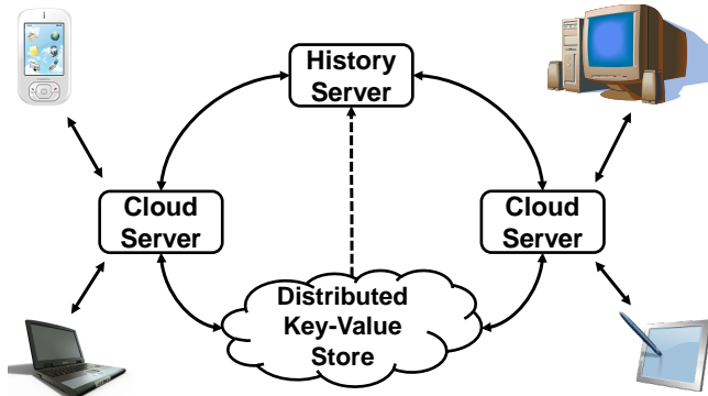
Fig. 1. Caelus architecture.
