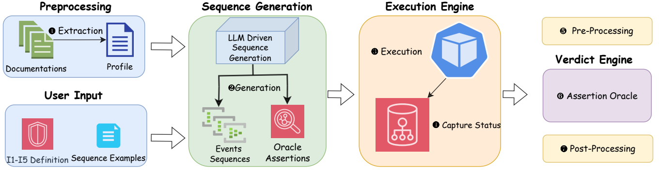
Figure 3: System overview of PORTA pipeline.
