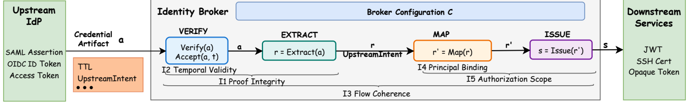
Figure 2: The four-stage trust translation pipeline and where each invariant (I1–I5) applies.
